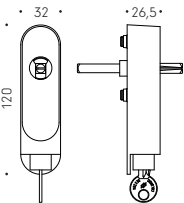
CD 02 DK LOCK Finishes: OL - CR - CM
